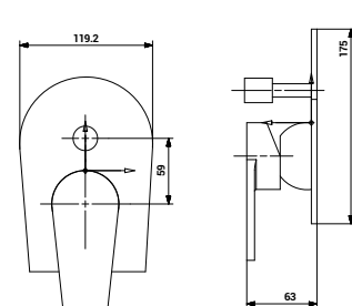
1530 Exposed Parts Kit of Single Lever Concealed Diverter Medium Body
