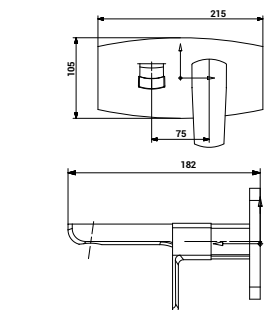
3018 Sink Cock Concealed Body Wall Mounted
