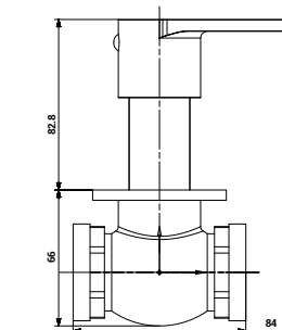
1209 Flush Cock in Ceramic Cartridge (25mm)
