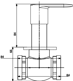
3109 Flush Cock in Ceramic Cartridge (25mm)
