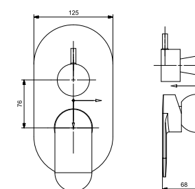
3135 Exposed Part Kit of Body Jet Single Lever Diverter
