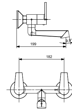
1514 Wall Mixer Non Telephonic Shower System
