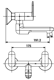
3114 Wall Mixer Non Telephonic Shower System
