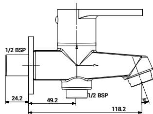
1507-1 2-Way Bib Cock Single Handle with wall Flange
