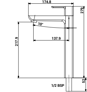
3029 Pillar Cock Extension Body
