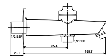
109 Bath tub Spout with Button Attachment for Telephone Shower
