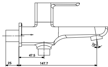
3007-1 2-Way Bib Cock Single Handle with wall Flange
