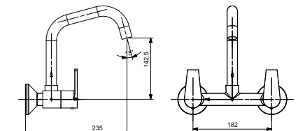
1524 Sink Mixer Long Swinging Spout Wall Mounted
