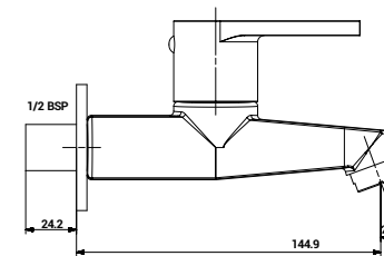
1225 Long Body Bib Cock with Wall Flange
