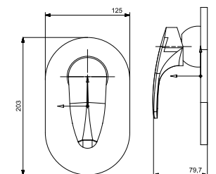
1236 Exposed Part Kit for Shower or Spout Single Lever Diverter
