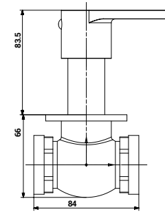
1513 Flush Cock with Adjustable Wall Flange (25 mm)
