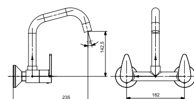
1224 Sink Mixer Long Swinging Spout W.M.
