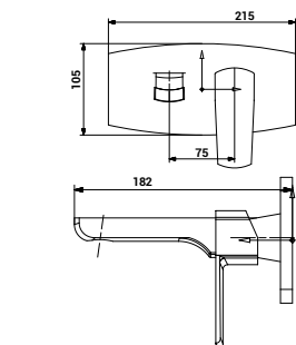
3019 Single Lever Sink Mixer Concealed Body
