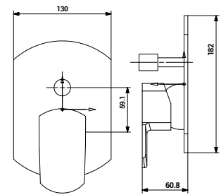
3028 Exposed Parts Kit of Single Lever Concealed High Flow Diverter 45 mm
