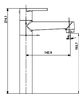
1529 Pillar Cock Extension Body
