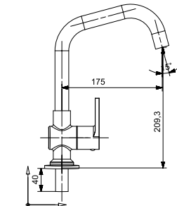
1210 Sink Cock with Extended Swinging Spout T.M.
