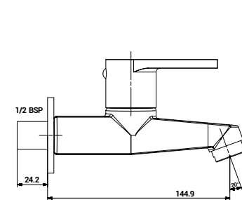
1525 Long Body Bib Cock with Wall Flange
