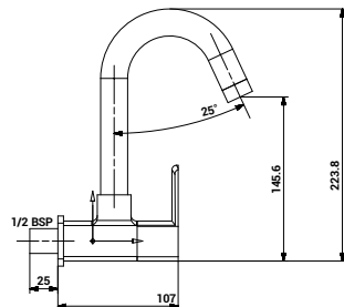
3004 Sink Cock with Swinging Spout Wall Mounted
