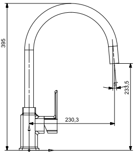
3032 Side Handle Single Lever Sink Mixer with Braided Hose
