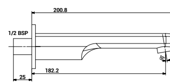
117 Bath Tub Spout with Wall Flange
