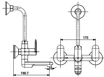
3115 Wall Mixer with Wall Bend Pipe
