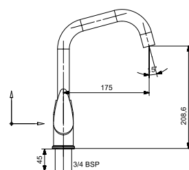
1222 Centre Hole Basin Mixer Extended Swinging Spout T.M.
