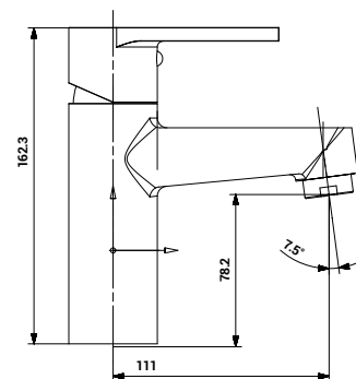
1526 Single Lever Basin Mixer
