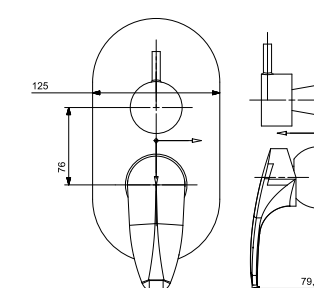
1235 Exposed Part Kit of Body Jet Single Lever Diverter
