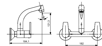
1523 Sink Mixer with Regular Swinging Spout Wall Mounted
