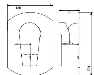
1536 Exposed Part Kit for Shower or Spout Single Lever Diverter
