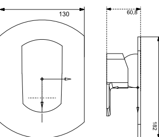
3036 Exposed Part Kit for Shower or Spout Single Lever Diverter
