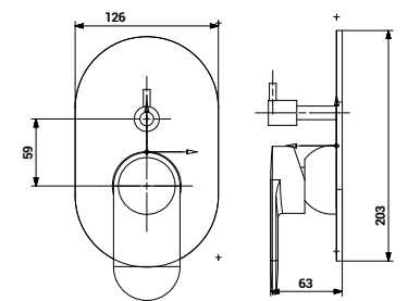
3133 Exposed Parts Kit of Single Lever High Flow Diverter (40 mm)
