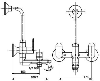
3117 Wall Mixer 3 in 1 with Provision for Both Shower
