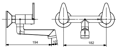
1214 Wall Mixer Non Telephonic Shower System
