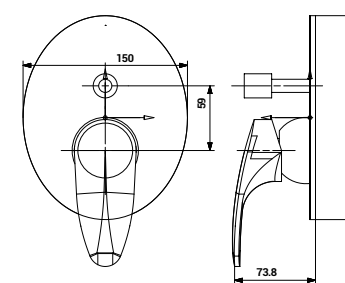
1228 Exposed Parts Kit of Single Lever Concealed High Flow Diverter 45 mm
