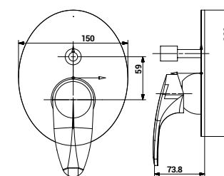
1234 Exposed Parts Kit of Single Lever High Flow Diverter (40 mm)
