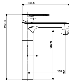
3127 Single Lever Basin Mixer with Extension Body
