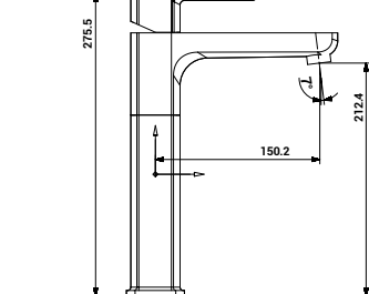
3027 Single Lever Basin Mixer with Extension Body
