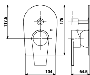
1534 Exposed Parts Kit of Single Lever High Flow Diverter (40 mm)
