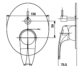
1233 Exposed Parts Kit of Single Lever High Flow Diverter (40 mm)
