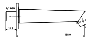
101 Bath Tub Spout with Wall Flange
