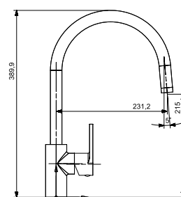
1532 Side Handle Single Liver Sink Mixer with Braided Hose
