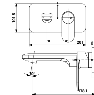
3119 Single Lever Sink Mixer Concealed Body
