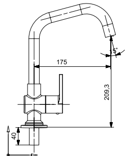
1510 Sink Cock with Extended Swinging Spout Table Mounted
