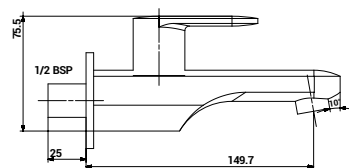
3125 Long Body Bib Cock with Wall Flange
