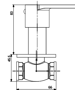
1208 Concealed Stop Cock with Adjustable Wall Flange (15mm )
