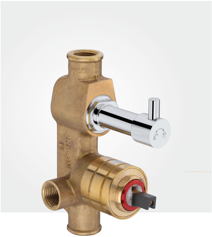
204 Single Lever High Flow Diverter Manual Closing System (40mm)
