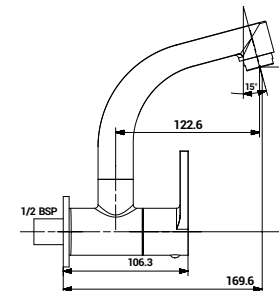
1204 Sink Cock with Swinging Spout Wall Mounted
