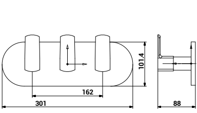
3031 4-Way Diverter for Concealed fitting Non-Return Valves
