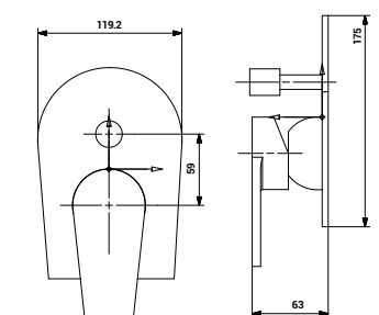
1528 Exposed Parts Kit of Single Lever Concealed High Flow Diverter 45 mm
