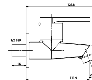
1202 Bib Cock with wall Flange
