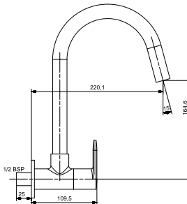
3111 Sink Cock with Extended Swinging Spout Wall Mounted
