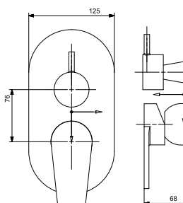
1535 Exposed Part Kit of Body Jet Single Lever Diverter
