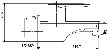
3102 Bib Cock with wall Flange
