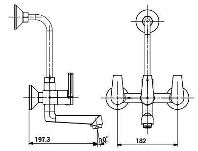
1515 Wall Mixer with Wall Bend Pipe
