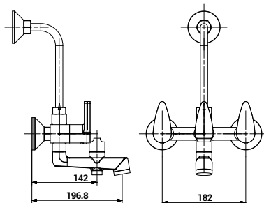
1217 Wall Mixer 3 in 1 with Provision for Both Shower
