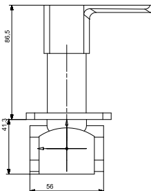
3008-1 Concealed Stop Cock with Adjustable Wall Flange (15mm)
