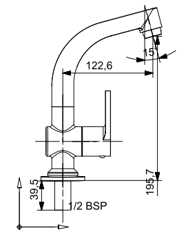
1203 Sink Cock with Swinging Spout Table Mounted
