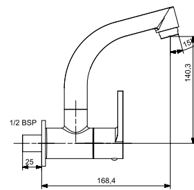
1504 Sink Cock with Swinging Spout Wall Mounted
