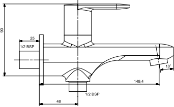
3107-1 2-Way Bib Cock Single Handle with wall Flange
