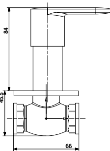
3108 Concealed Stop Cock with Adjustable Wall Flange (15mm )
