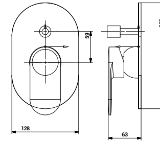
3128 Exposed Parts Kit of Single Lever Concealed High Flow Diverter 45 mm
