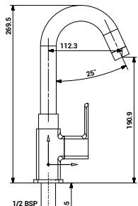
3003 Sink Cock with Swinging Spout Table Mounted
