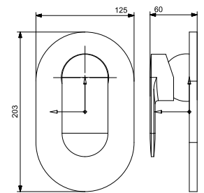
3136 Exposed Part Kit for Shower or Spout Single Lever Diverter
