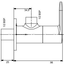
3105 Angular Stop Cock with Wall Flange
