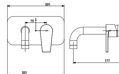
1519 Single Lever Sink Mixer Concealed Body
