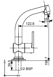
1503 Sink Cock with Swinging Spout Table Mounted
