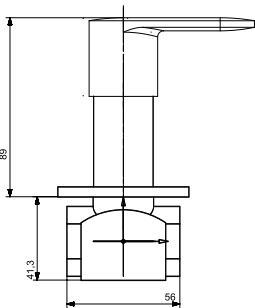
3108-1 Concealed Stop Cock with Adjustable Wall Flange (15mm)
