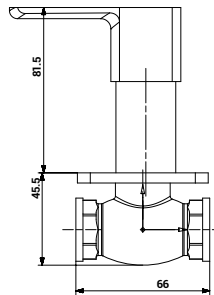
3008 Concealed Stop Cock with Adjustable Wall Flange (15mm )
