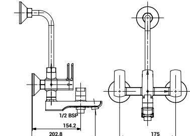
3017 Wall Mixer 3 in 1 with Provision for Both Shower
