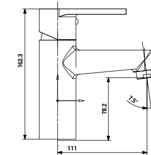
1226 Single Lever Basin Mixer
