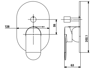
3130 Exposed Parts Kit of Single Lever Concealed Diverter Medium Body
