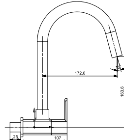
3011 Sink Cock with Extended Swinging Spout W.M.
