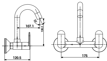
3123 Sink Mixer with Regular Swinging Spout Wall Mounted
