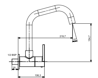
1211 Sink Cock with Extended Swinging Spout W.M.
