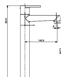
1221 Pillar Cock Extra Extension Body
