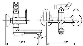
3116 Wall Mixer with Crutch for Arrangement of Telephone Shower
