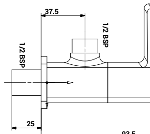
3005 Angular Stop Cock with Wall Flange
