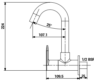
3104 Sink Cock with Swinging Spout Wall Mounted
