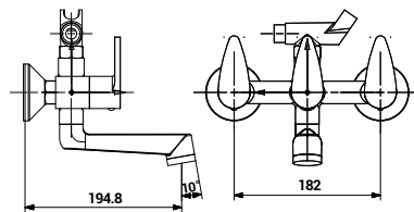
1216 Wall Mixer with Crutch for Arrangement of Telephone Shower
