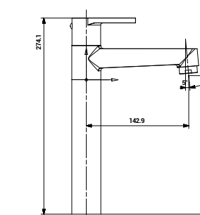
1229 Pillar Cock Extension Body
