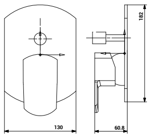
3034 Exposed Parts Kit of Single Lever High Flow Diverter (40 mm)
