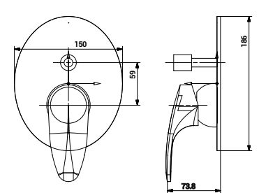
1230 Exposed Parts Kit of Single Lever Concealed Diverter Medium Body
