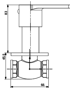
1508 Concealed Stop Cock with Adjustable Wall Flange (15mm )
