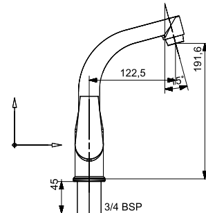
1506 Centre Hole Basin Mixer Regular Spout with 450mm Hose
